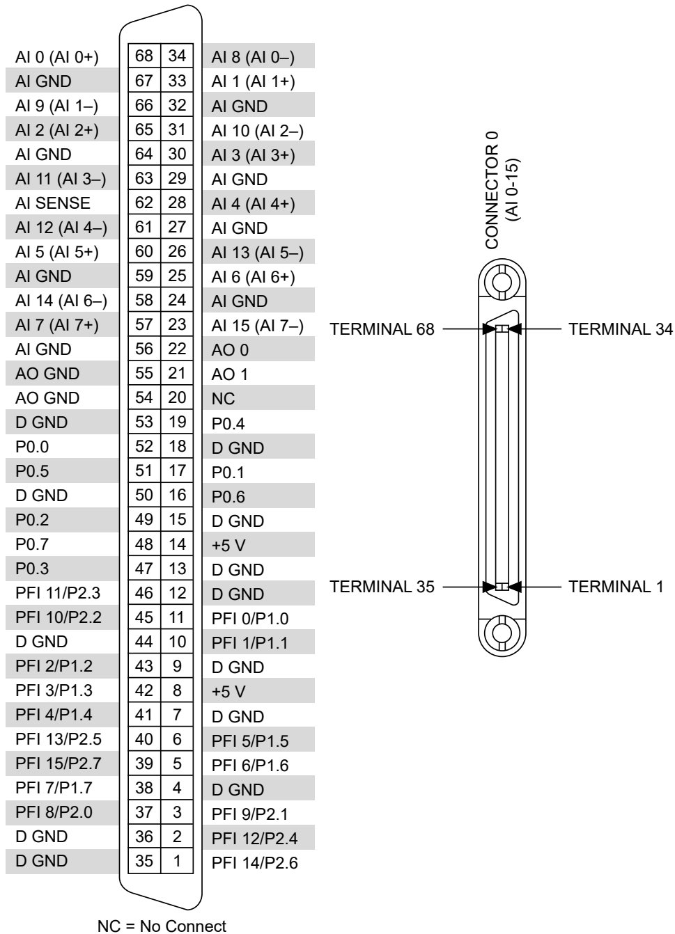
Figure 1. PXIe-6321 Pinout
